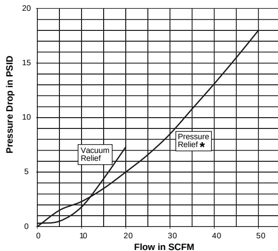
H1 and HM1 Pressure-Vacuum Relief Valve
