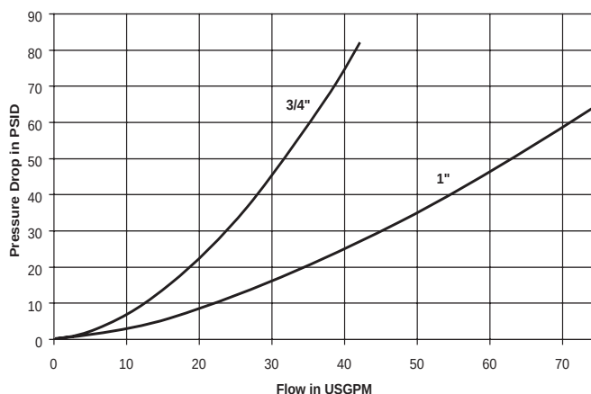
4000 Series (3/4\" & 1\") Test Fluid: Oil - 200 SUS
